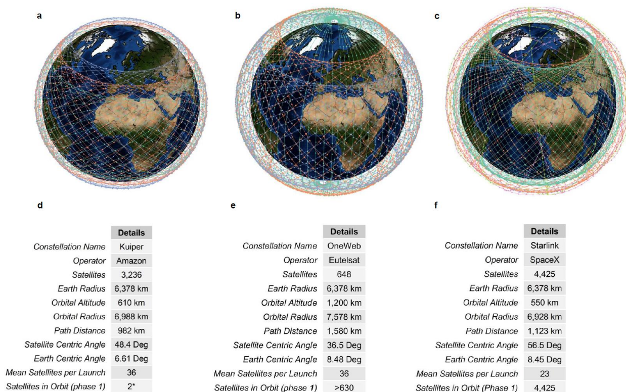
Fig. 1 | Technical details of the constellations as at December, 2023. a , Amazon's Kuiper is in a testing phase having launched only two prototype satellites (KuiperSat-1 and KuiperSat-2), and are yet to launch any of the planned 3,236 phase 1 satellites (December 2023), b , OneWeb has deployed 98% of the 648 phase 1 satellites (December 2023), c , SpaceX Starlink has launched 100% of the 4,425 phase 1 satellites [23], [24], [25] (December 2023).
