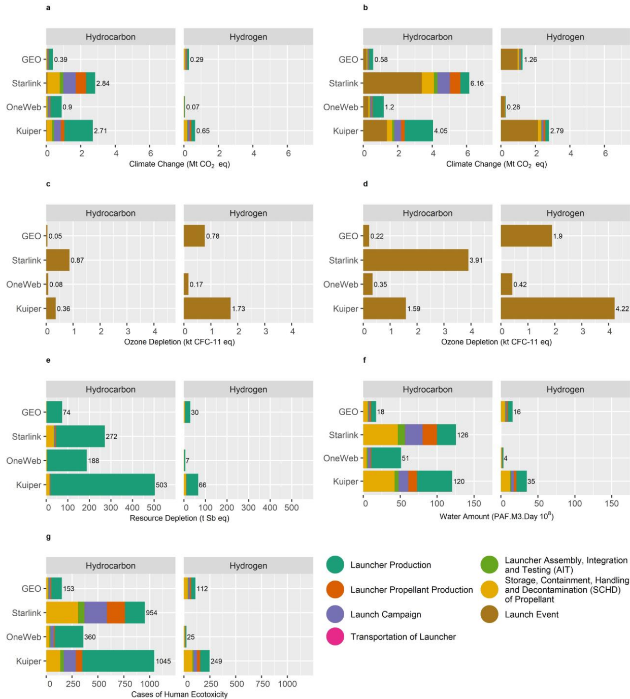
Fig. 4 | Key constellations by environmental impact category. a , Climate change impacts (baseline), b , Climate change impacts including NIEs (worst-case), c , Ozone depletion (baseline), d , Ozone depletion including NIEs (worst-case), e , Resource depletion, f , Freshwater ecotoxicity, g , Human toxicity.
