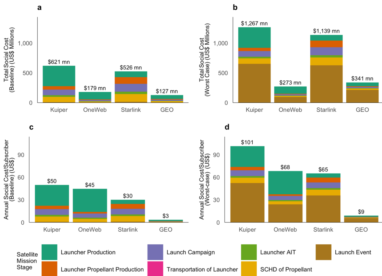
Fig. 5 | Social cost of carbon. a , The total SCC of the emissions baseline over a five (LEO) and fifteen (GEO)-year time horizon, b , The total SCC of the emissions worst-case, c , The Annualized SCC per subscriber for the emissions baseline, d , The Annualized SCC per subscriber for the emissions worst-case over the time horizon.
