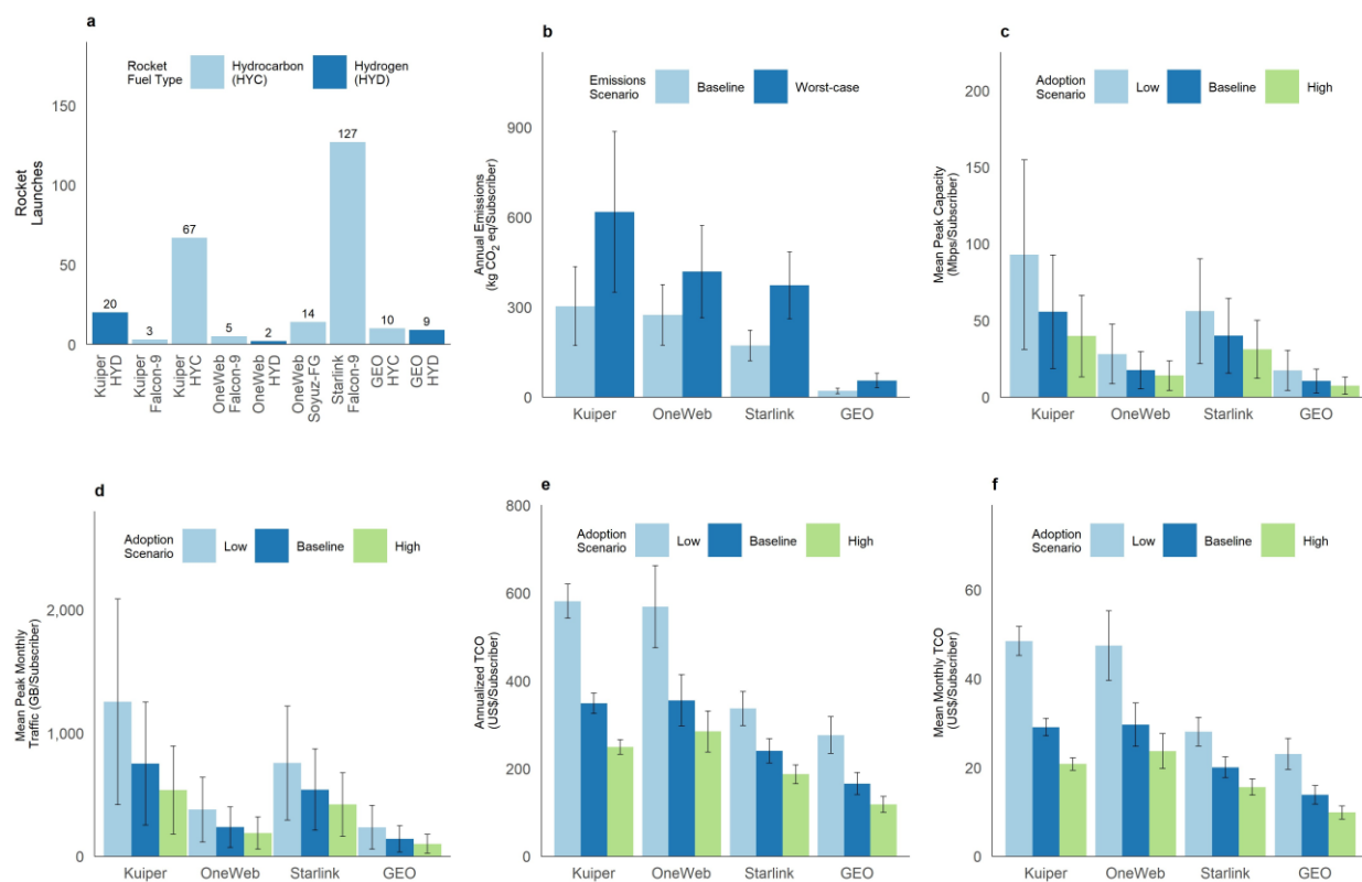
Fig. 3 | Constellation Metrics. a , Quantity of rocket launches by constellation and rocket fuel-type, based on information as of December 2023. We use generic hydrogen (HYD) and hydrocarbon (HYC) rocket vehicles when the exact launcher is not in the SSSD database or the rocket type is unknown (via a 50-50 split). In total for this evaluation, 63% of assessed LEO launches are based on a modeled rocket, 36% utilize a generic rocket for a known launcher, and only 2% utilize a generic rocket for an unknown launcher. b , Equivalent annual emissions estimated per subscriber for each constellation, given the baseline versus the worst-case emissions outcome, with Confidence Intervals (CIs) representing low and high subscriber adoption scenarios, c , The estimated mean provided peak data rate with CIs representing 1 Standard Deviation (SD) in mean capacity for each adoption scenario, d , Potential peak monthly traffic per subscriber estimated with CIs representing 1 SD in monthly traffic for each adoption scenario, e , The estimated
